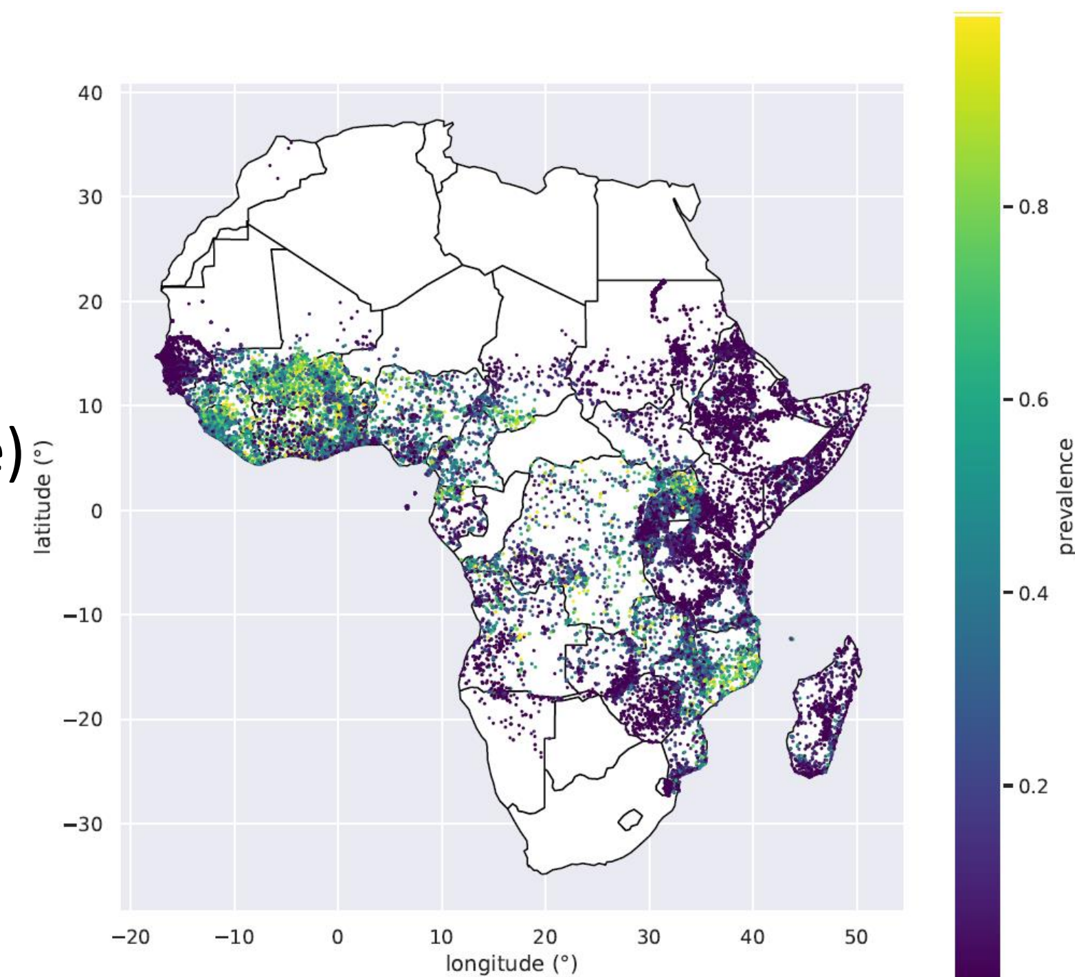
Fig.2 Malaria prevalence, used as training data for the model.
