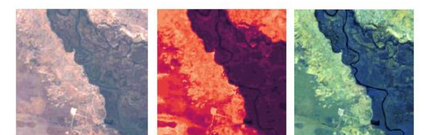
Fig.3 Example of different Landsat 8 bands from one location. From left to right: RGB bands, Infrared bands, Thermal band.
