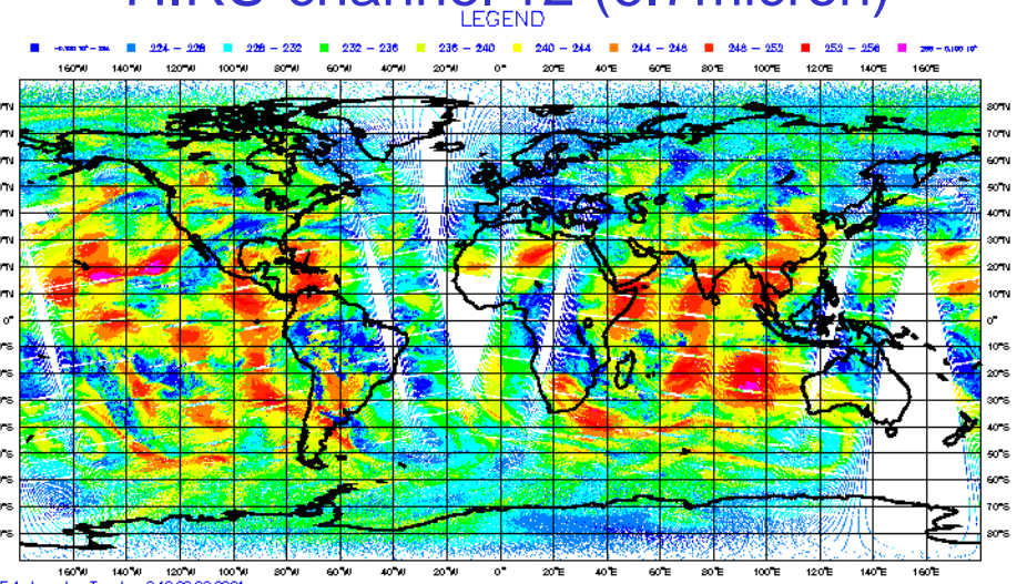
HIRS-channel 12 (6.7micron)
