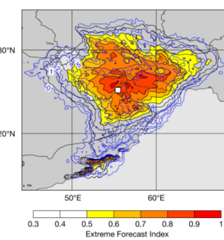
EFI and SOT. The Extreme Forecast Index (EFI – shading) and Shift of Tails (SOT – contours) for 24-hour rainfall on 16 April in the forecast from 10 April 00 UTC.
