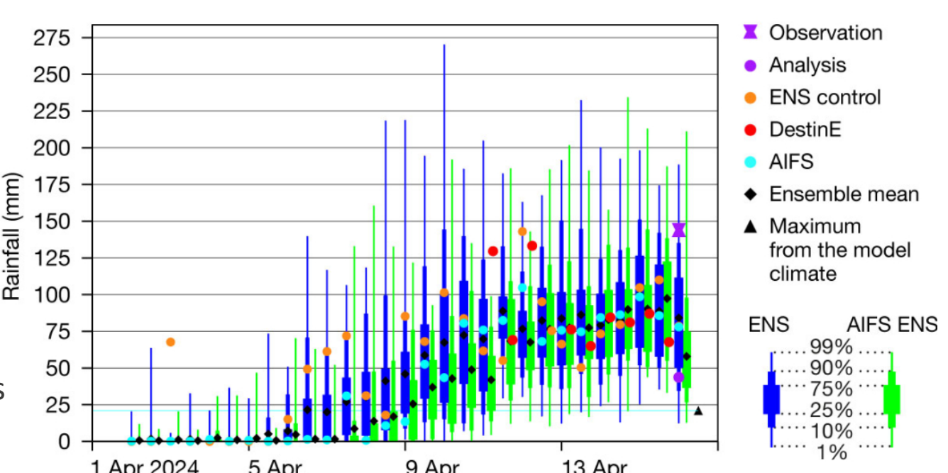
Forecast evolution plot for Dubai. The plot shows the evolution of 24-hour rainfall forecasts on 16 April over the grid box including Dubai. The model climate is about zero precipitation, with a maximum of less than 25 mm based on 1,800 forecasts (marked by the black triangle).
