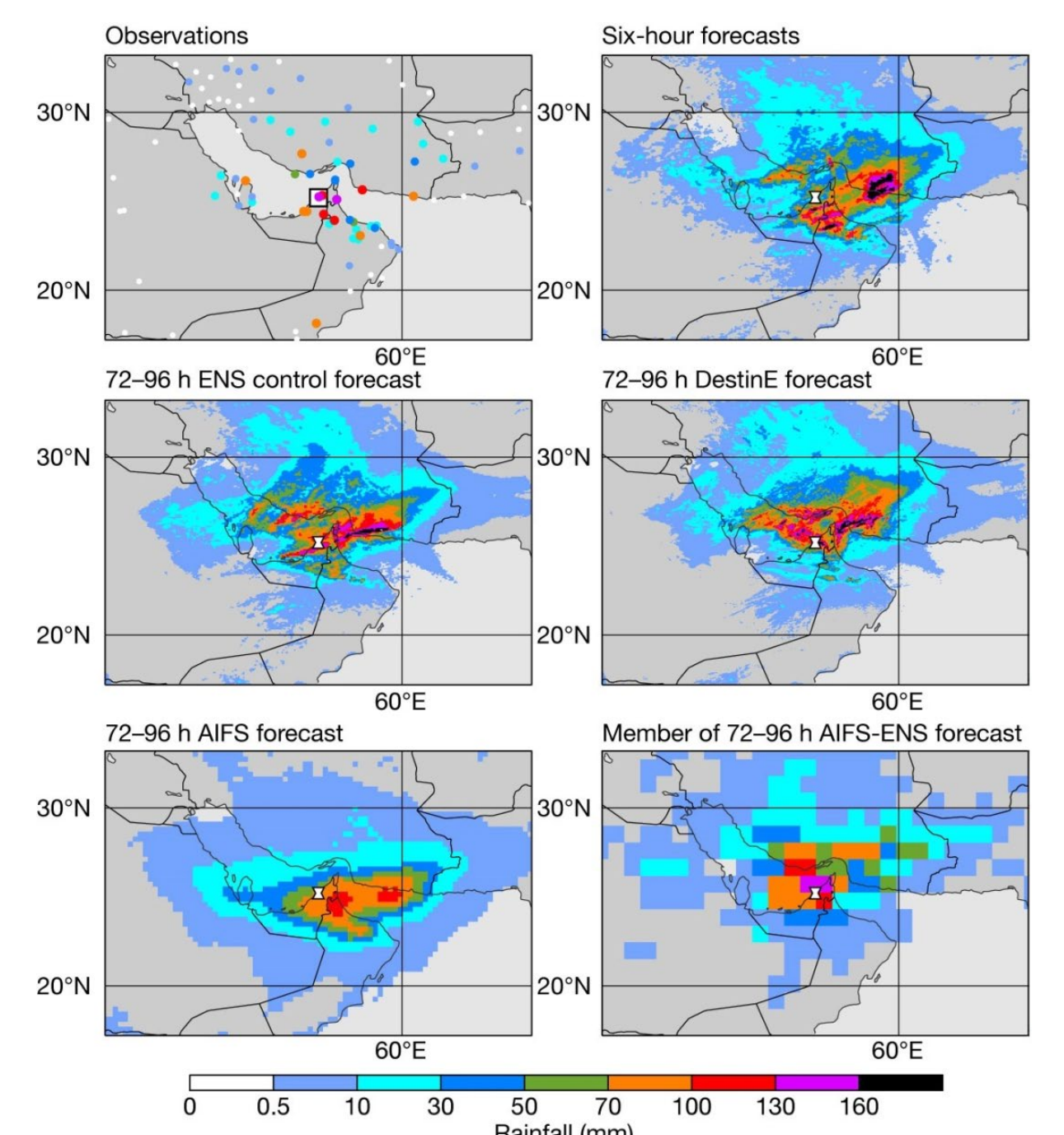
Twenty-four-hour rainfall from 16 April 00 UTC to 17 April 00 UTC. The charts show observations (top left); concatenated 6-hour forecasts (top right); 72–96 h forecasts from the ENS control at 9 km (middle left), DestinE at 4.4 km (middle right), and the AIFS at 28 km (bottom left); and the first perturbed member from the AIFS-ENS at 111 km (bottom right).
