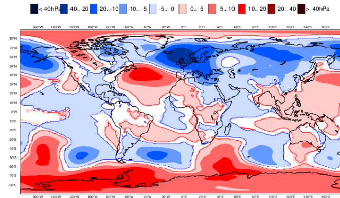
ECMWF EPS-Monthly Forecasting System mean SLP anomaly Forecast start reference is 09-12-2019 ensemble size = 51 , climate size = 660 Day 1-7 09-12-2019/TO/15-12-2019 Shaded areas significant at 10% level Contours at 1% level
