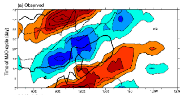
Composites of SST anomalies (contours) and OLR (colours) of MJO events. SST and convection are in quadrature.
