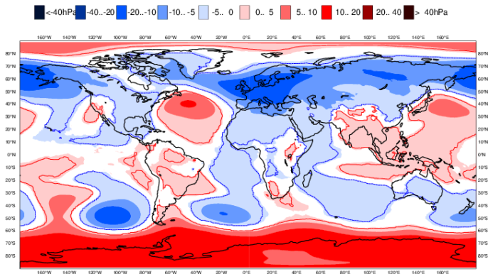
ECMWF EPS-Monthly Forecasting System mean SLP anomaly Forecast start reference is 09-12-2019 ensemble size = 51 , climate size = 660 Day 8-14 09-12-2019/TO/15-12-2019 Shaded areas significant at 10% level Contours at 1% level
