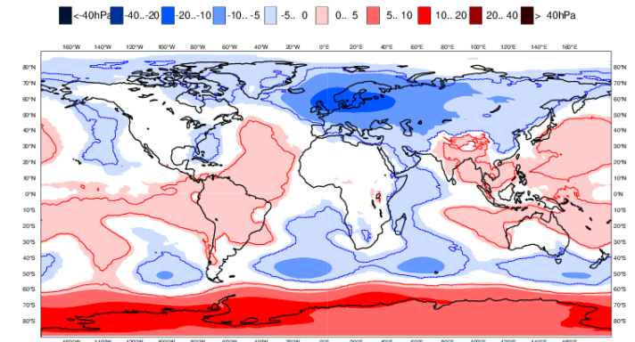
ECMWF EPS-Monthly Forecasting System mean SLP anomaly Forecast start reference is 25-11-2019 ensemble size = 51 , climate size = 660 Day 15-21 09-12-2019/TO/15-12-2019 Shaded areas significant at 10% level Contours at 1% level
